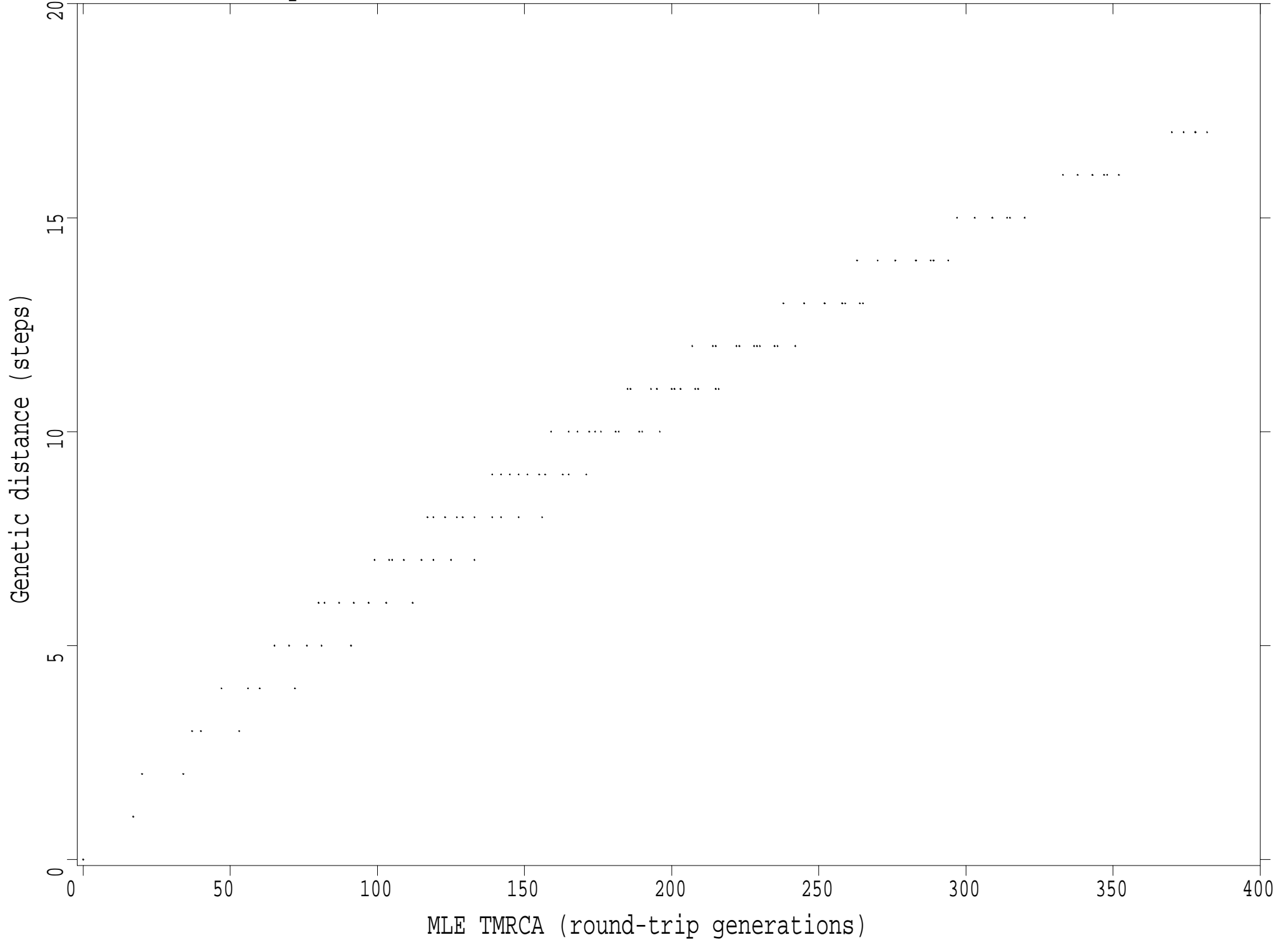
TMRCA vs stepwise distance for 25 loci with 0.0023 mutation rate
